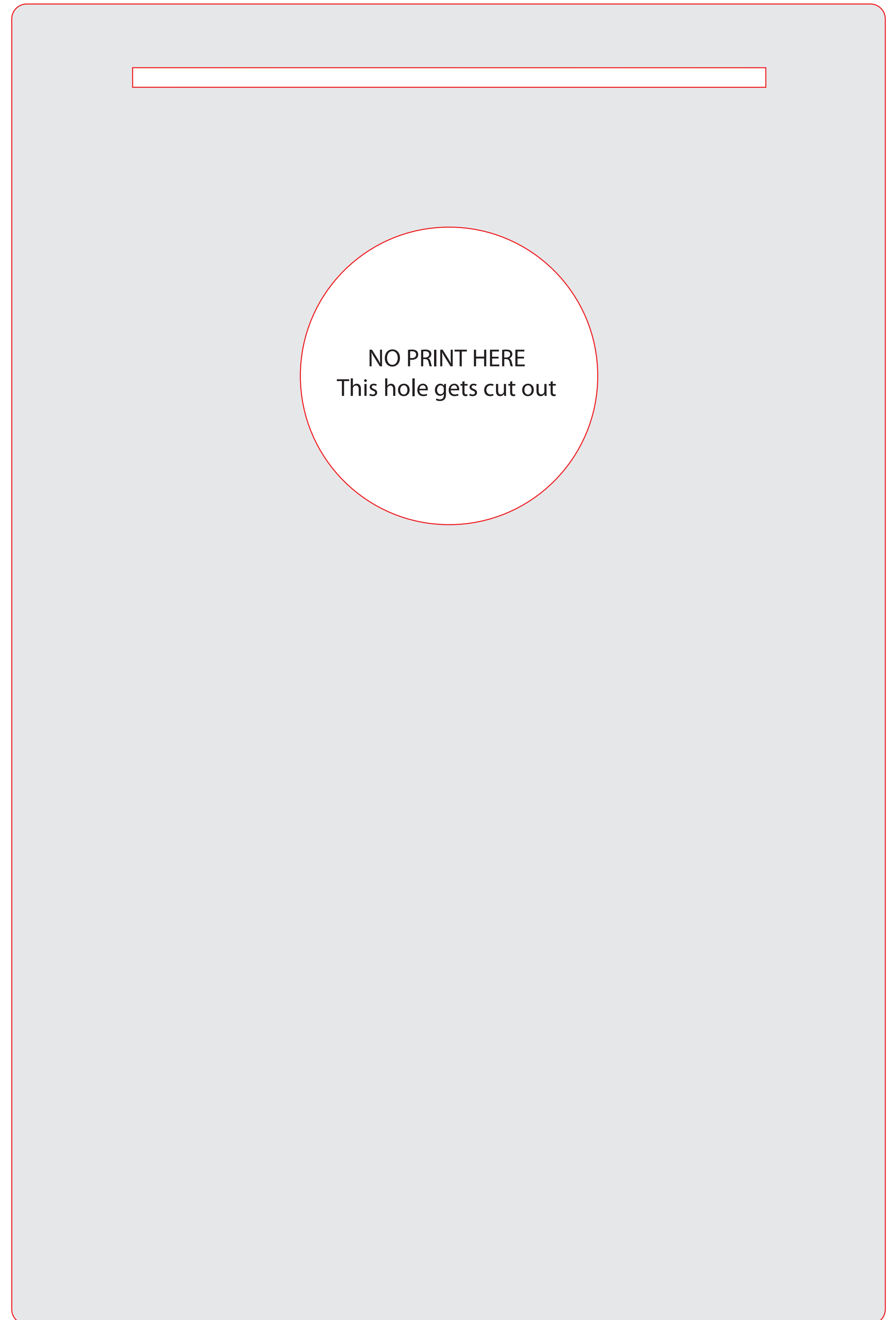
Cornhole Top
